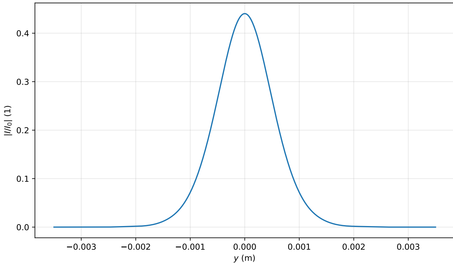
Intensity profile I(x=0, y, z=3.662)/I_0 , P_{in}=0.5P_{cr} , artificial time
